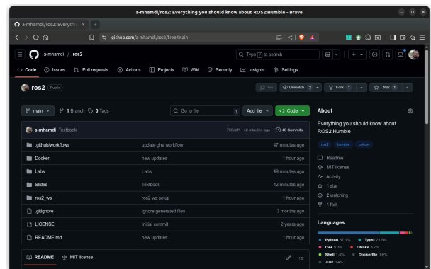
Figure 6: GitHub repository
