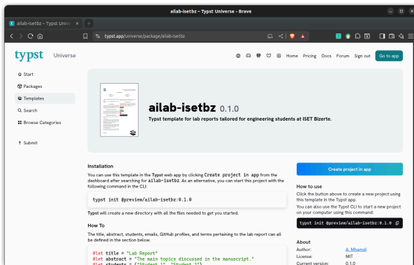
Figure 4: Typst app
