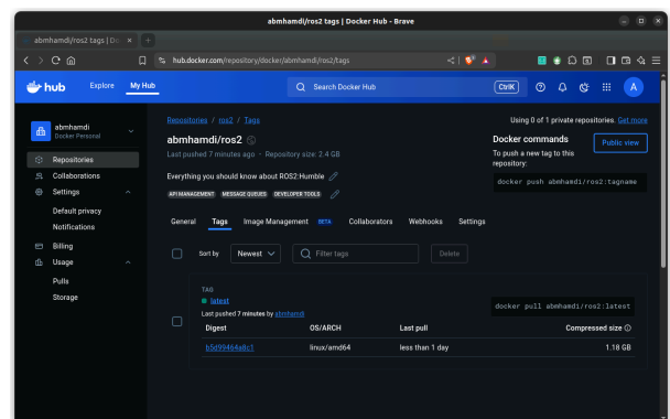
Figure 7: Docker image
