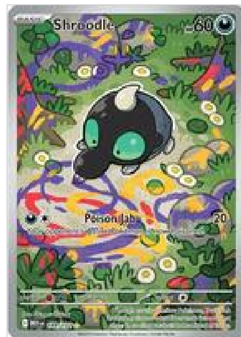
Shroodle - 149/132
