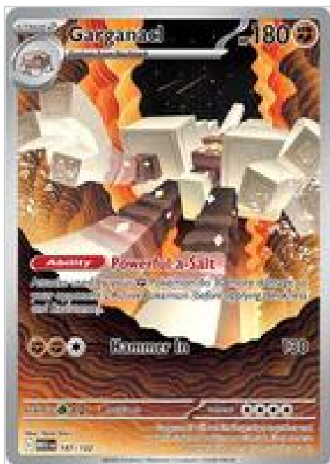
Garganacl - 147/132
