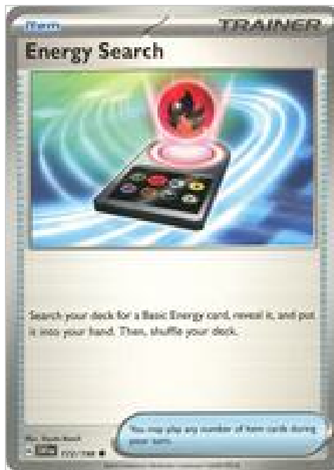
Energy Search
