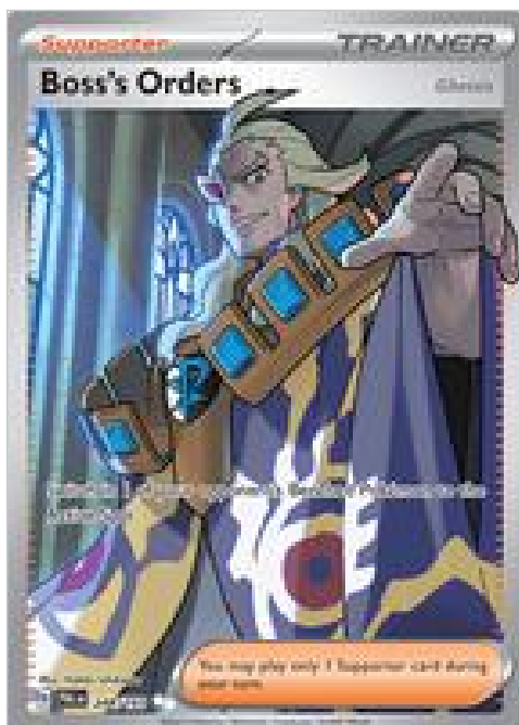
Boss's Orders - 248/193
