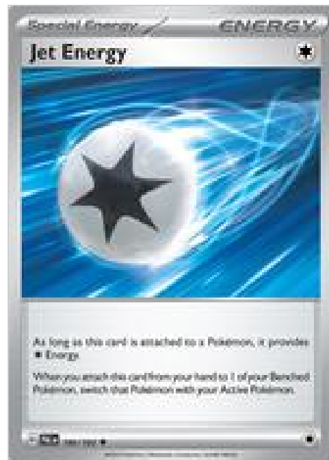
Jet Energy
