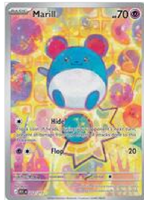
Marill - 232/217
