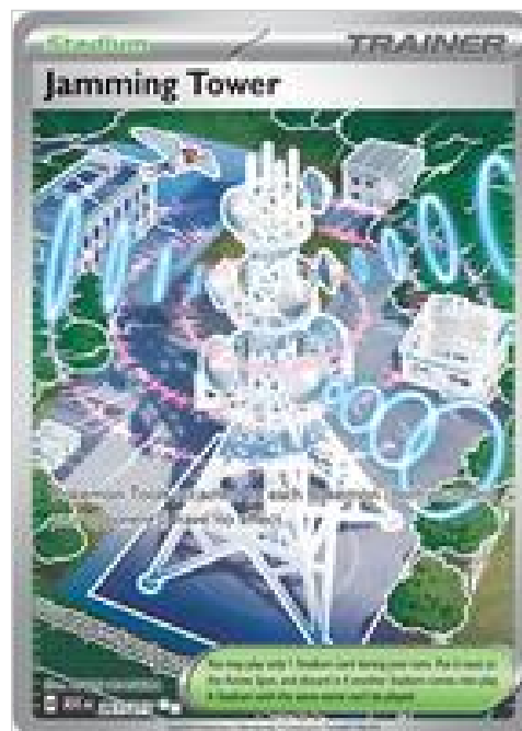
Jamming Tower - 261/217
