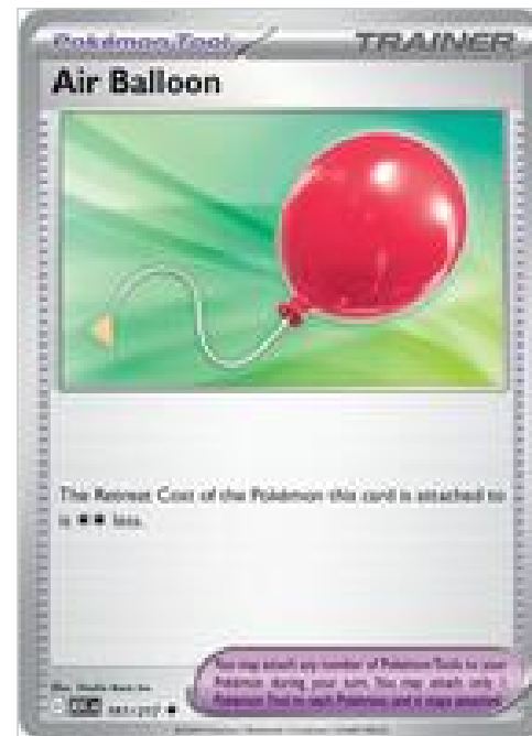
Air Balloon - 181/217
