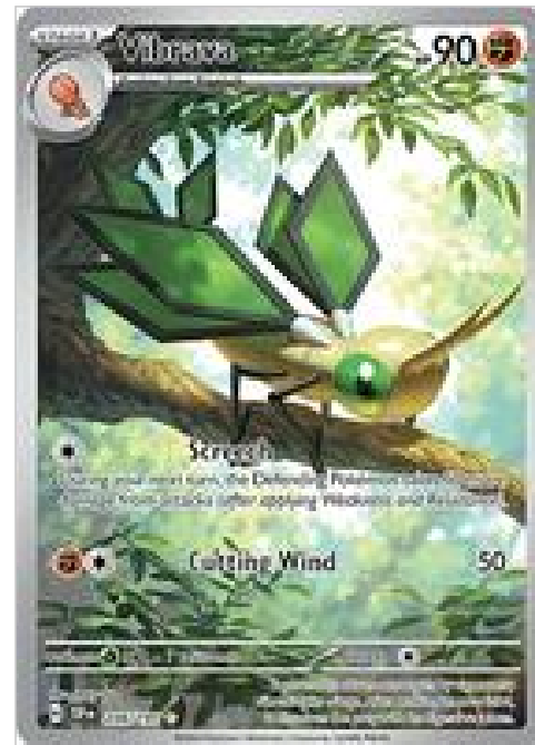
Vibrava - 206/191
