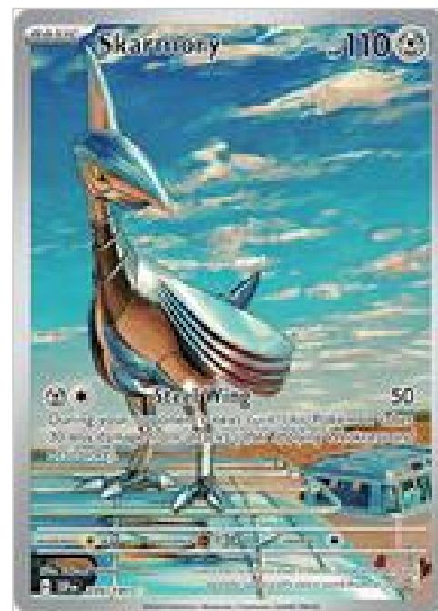
Skarmory - 209/191
