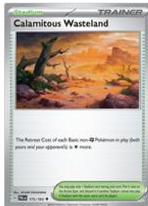
Calamitous Wasteland - 175/193
