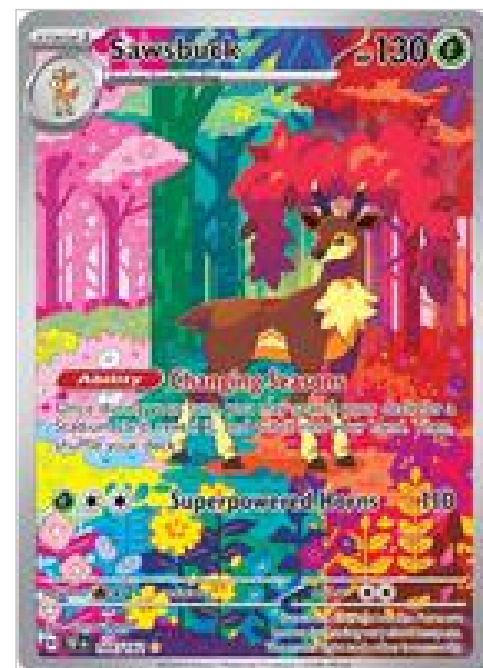
Sawsbuck - 166/162
