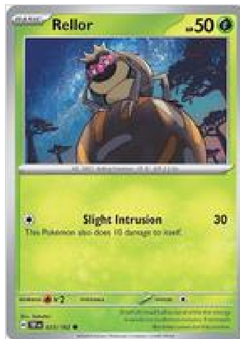
Rellor
