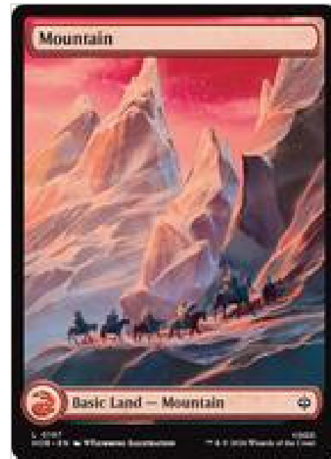
Mountain (0197)
