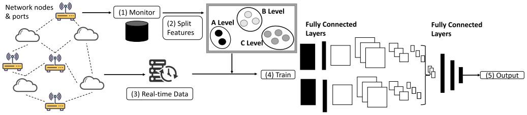
(a) Chen et al. DDoS Multi-Channel Convolutional Neural Network Incremental (MC-CNN) Learning Model [29]: Chen et al. implemented a multi-channel incremental network that monitored network traffic and packets, inputting the data into a database (represented as a black cylinder). Features are split into traffic, packet, and host level, which are represented through the A, B, C levels. Then the real-time data from the network along with the partitioned features are passed into a multi-channel CNN where the top branch accepts traffic features and the lower branch takes in packet features. The top layer undergoes pooling to reduce parameter complexity in the fully connected layer. The top and bottom branches are combined and passed to the fully connected layers and a final prediction is outputted.
