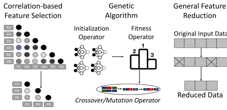
(a) Correlation-based feature selection [92]: The features are lined up on the horizontal and vertical axes of the correlation map. The method chooses features that are highly correlated with a class, but not correlated with each other. Genetic algorithm [58]: Ganapathy et al. identified a trending feature selection method using genetic algorithm that uses a fitness function and a decision tree where features are removed and model fitness so the optimal feature set is obtained.
