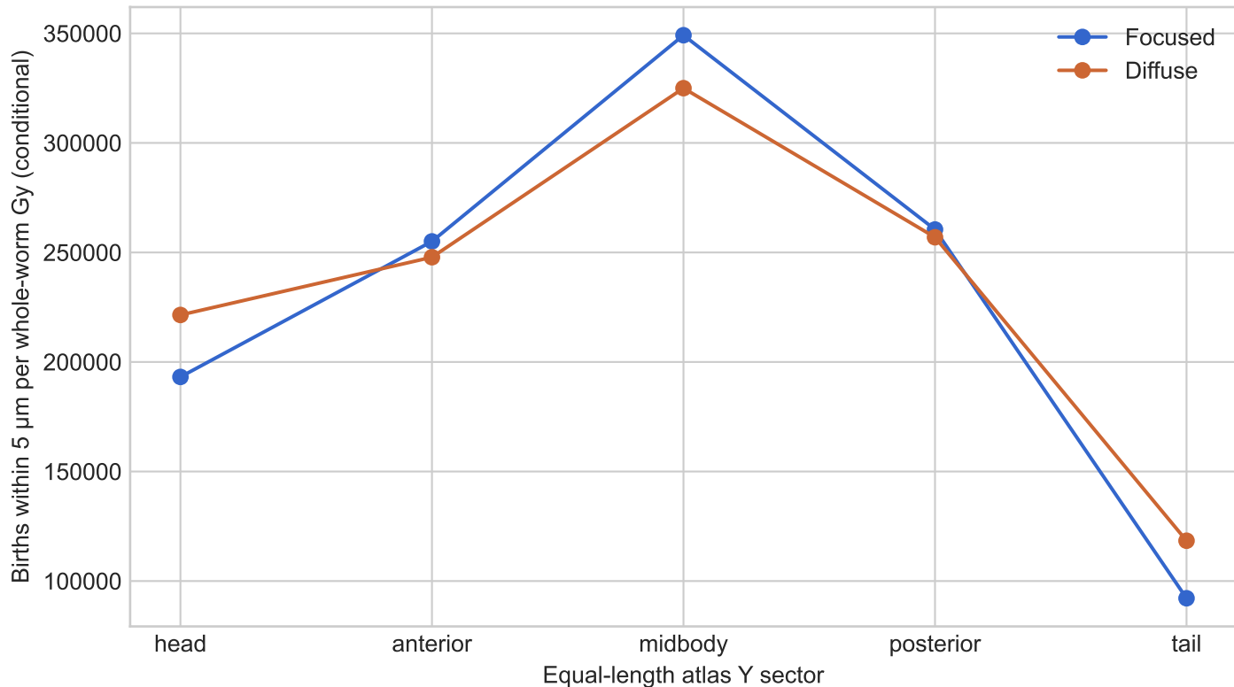
Longitudinal distribution of near-neural electron births
