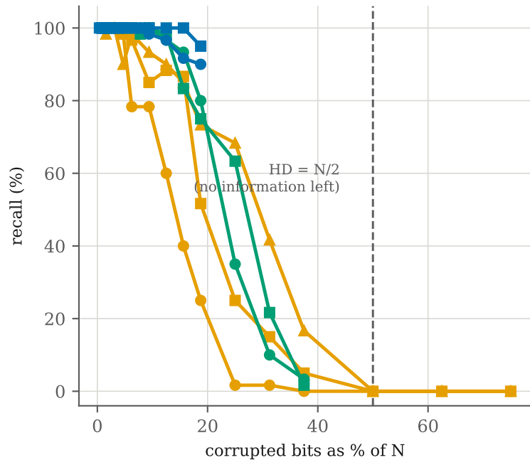
Relative corruption
