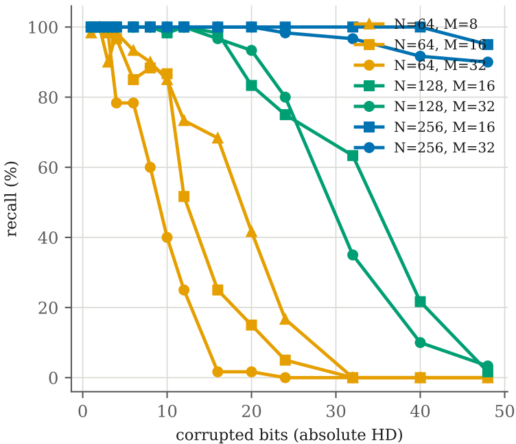
Absolute corruption
