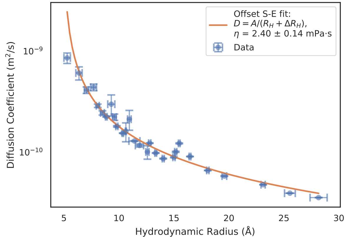
Diffusion Coefficient vs Hydrodynamic Radius
