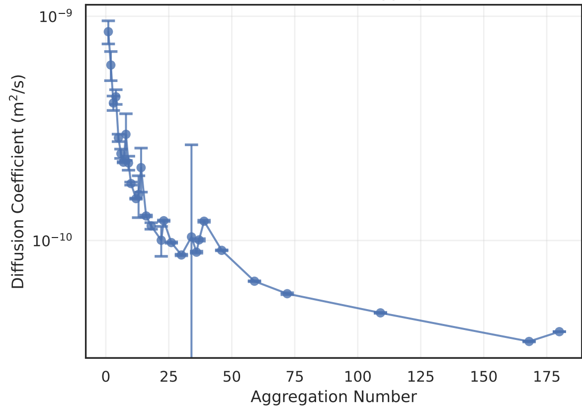
Diffusion Coefficient vs Aggregate Size
