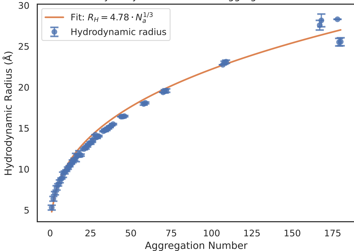
Hydrodynamic Radius vs Aggregate Size
