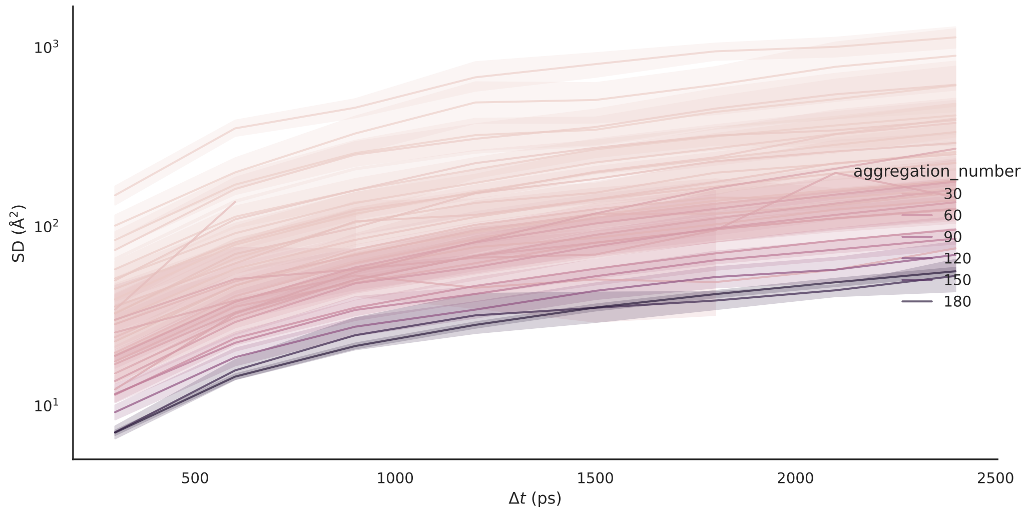
Squared Displacement vs Time by Aggregate Size
