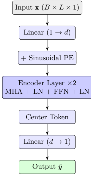
(a) Transformer TEQ
