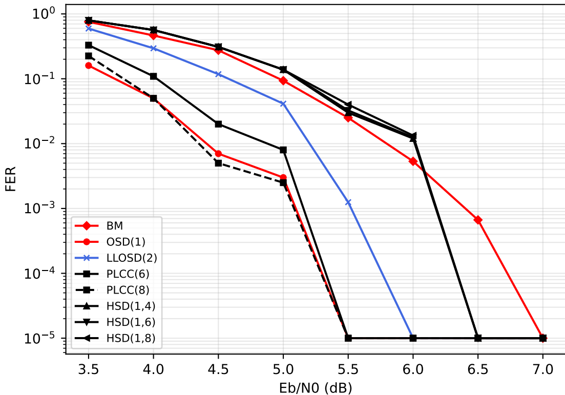
Fig. 9: (255, 223) BCH (fixed HSD)
