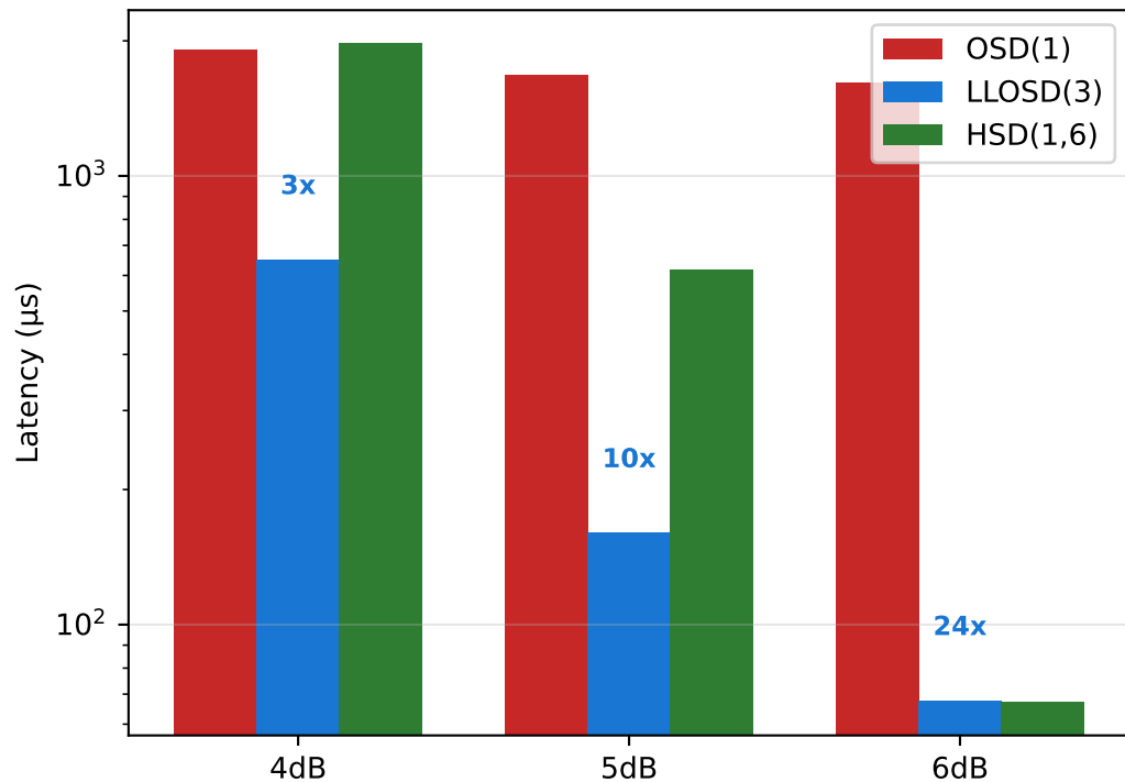
(127, 99) BCH — per-frame decoding latency
