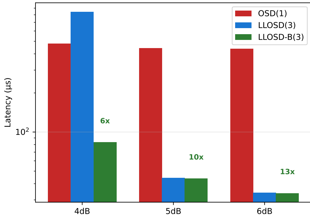
(63, 45) BCH — per-frame decoding latency
