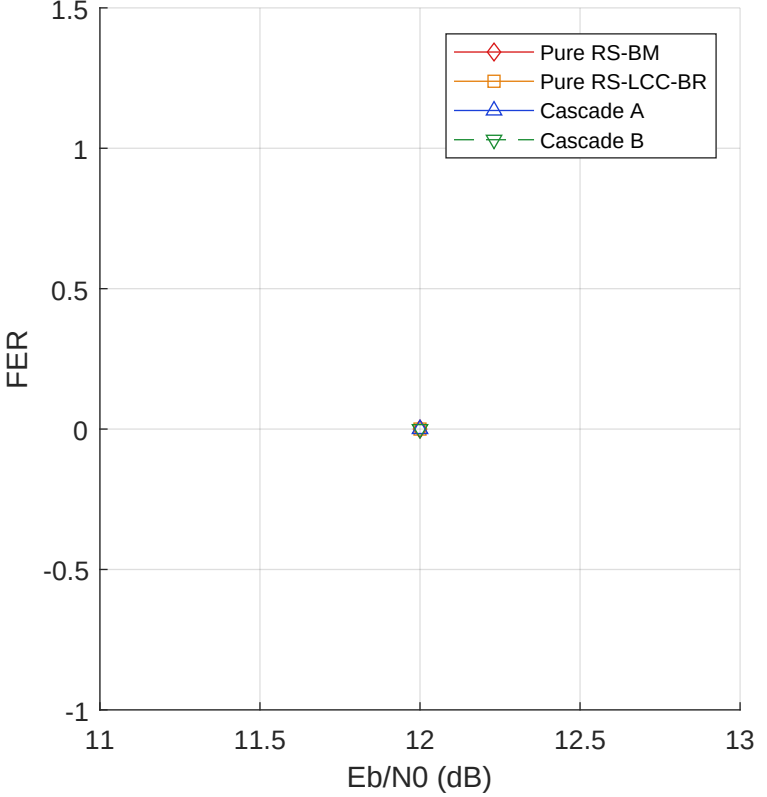
n255_B: RS(255,235) + BCH(255,247), total rate = 0.8927
