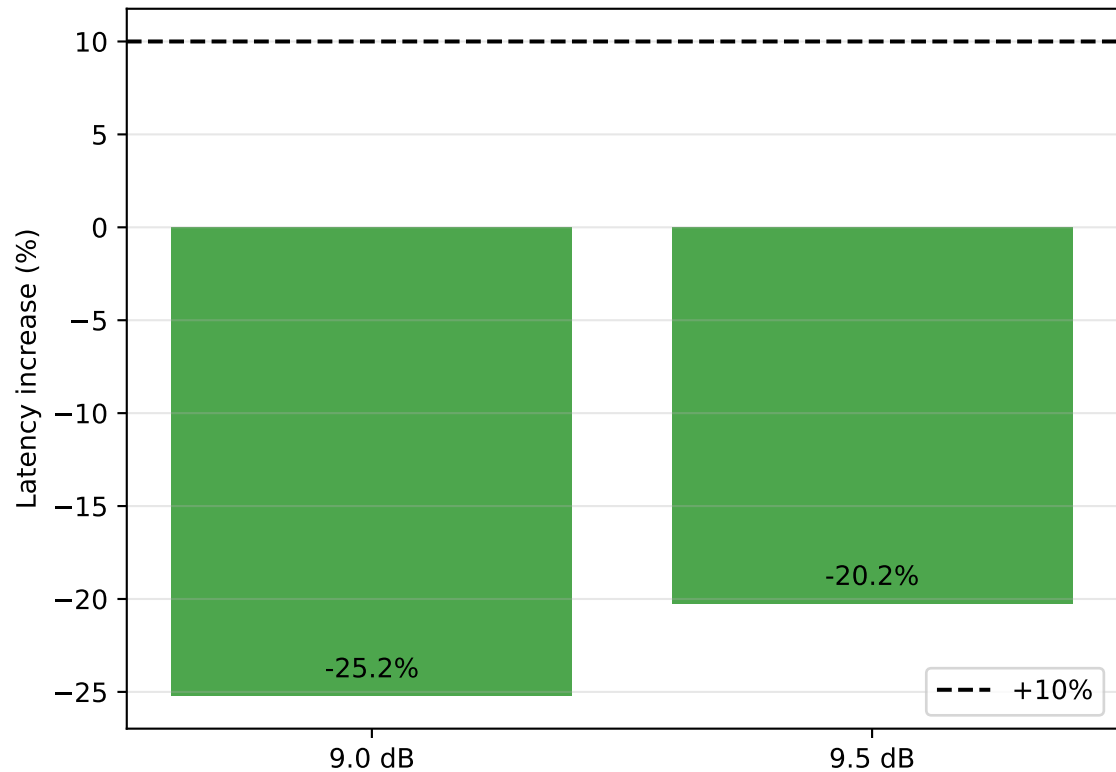
Case (b): Cascade vs Pure RS-LCC-BR (soft baseline)
