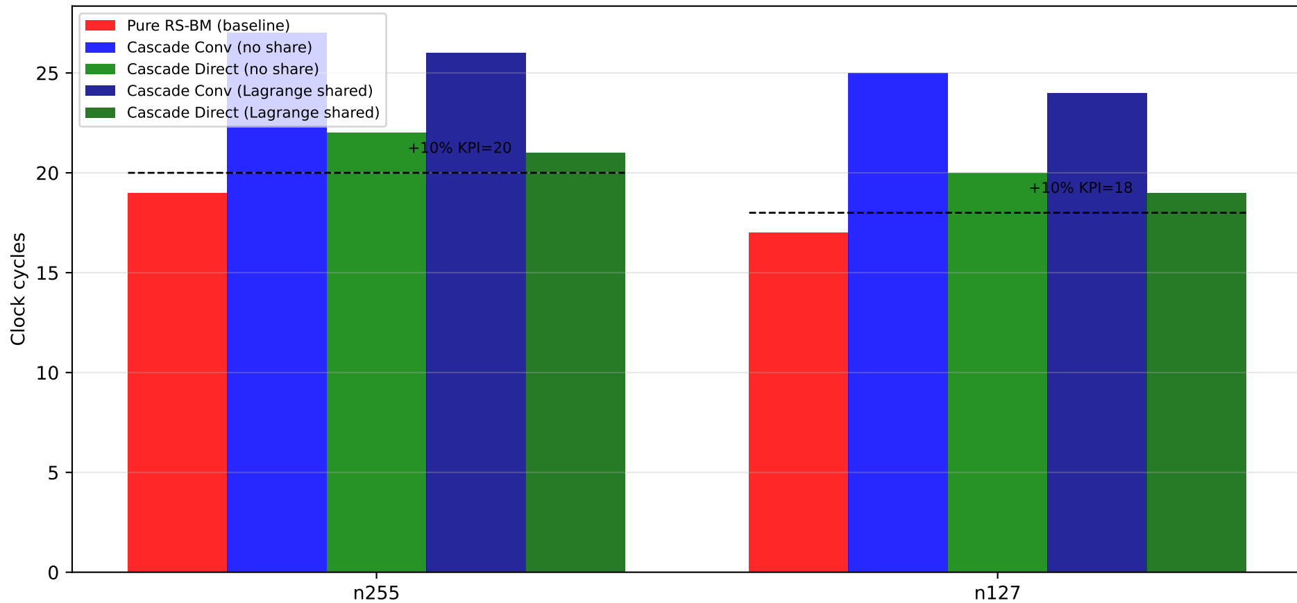
Cascade latency: clock cycles vs Pure RS-BM baseline
