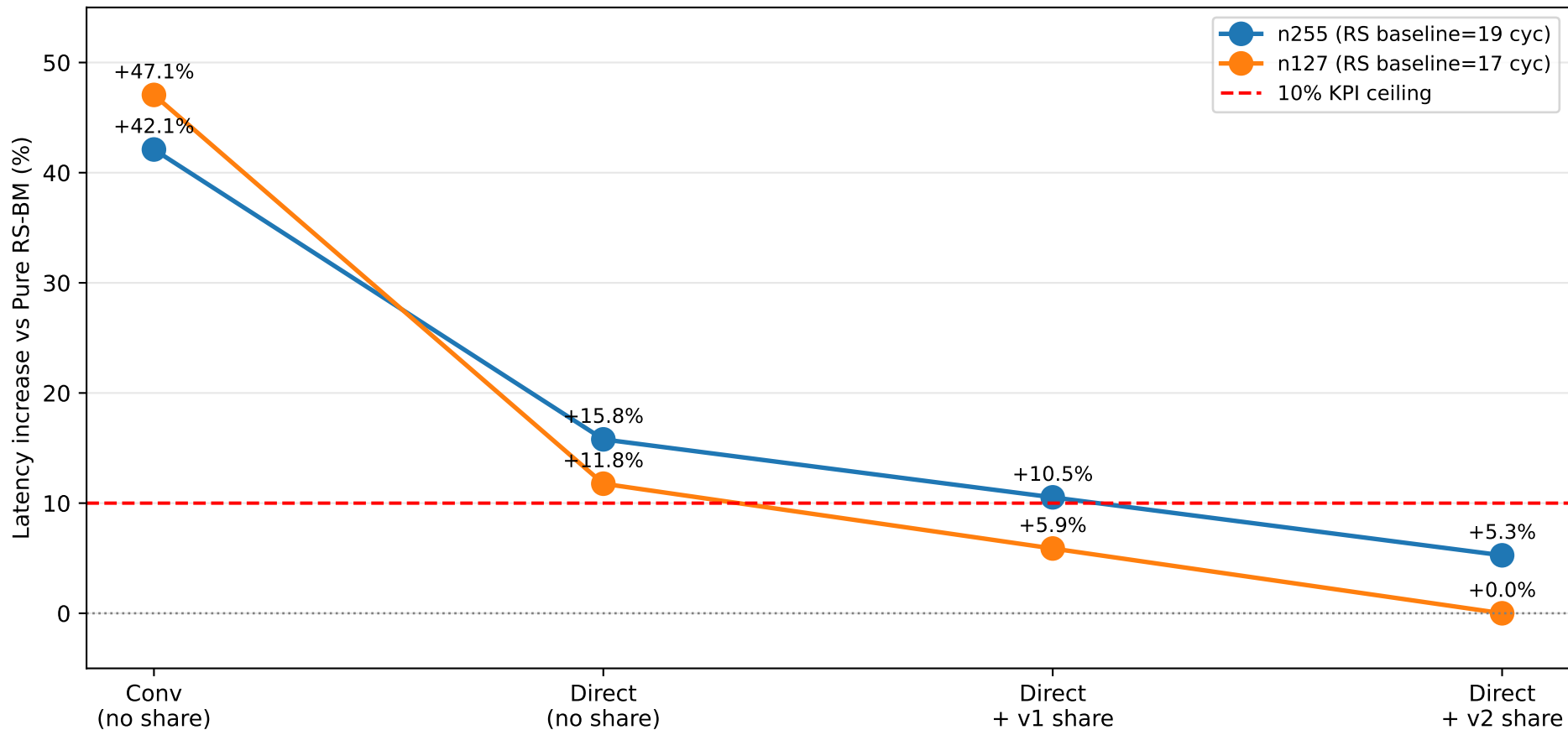
Cascade latency evolution: optimizations from Conv to Direct v2 share
