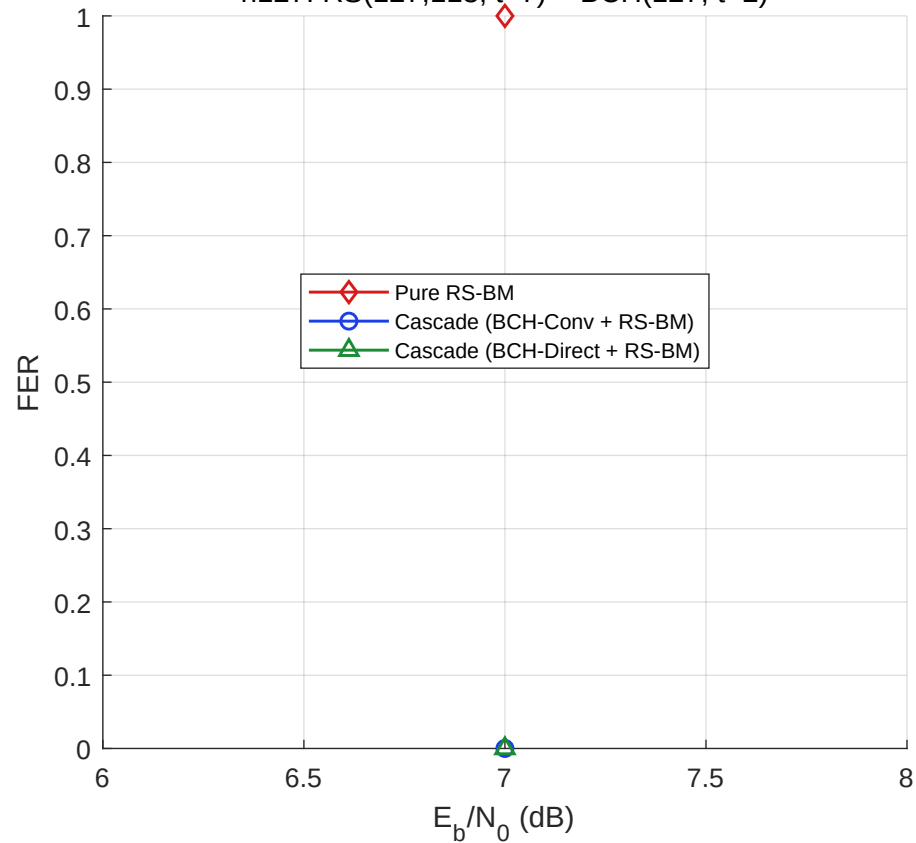
n127: RS(127,113, t=7) + BCH(127, t=2)
