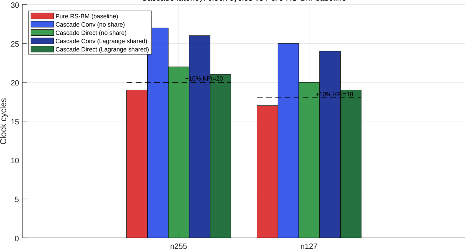
Cascade latency: clock cycles vs Pure RS-BM baseline
