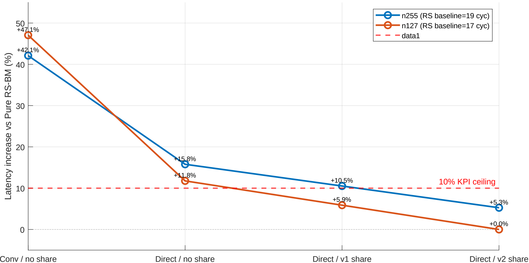
Cascade latency evolution: Conv to Direct v2 share
