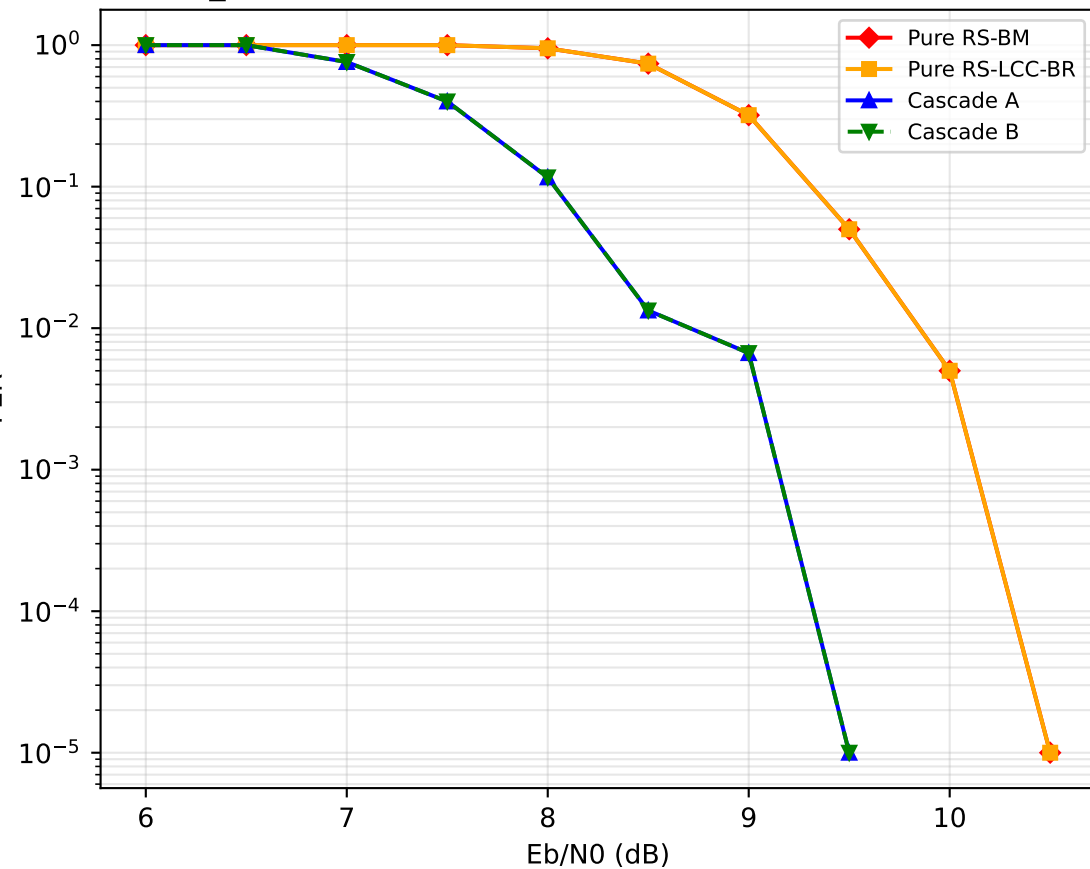
n255_A: RS(255,239) + BCH(255,239), total rate = 0.8784
