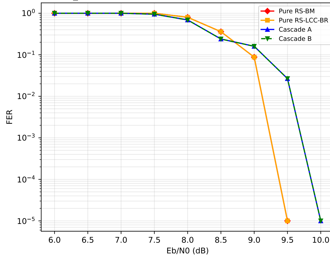
n255_B: RS(255,235) + BCH(255,247), total rate = 0.8927
