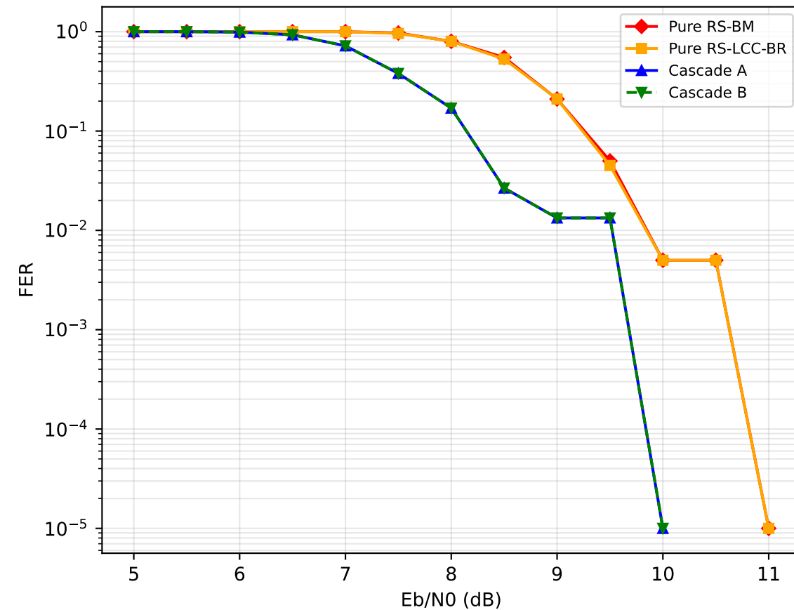
n127: RS(127,119) + BCH(127,120), total rate = 0.8854
