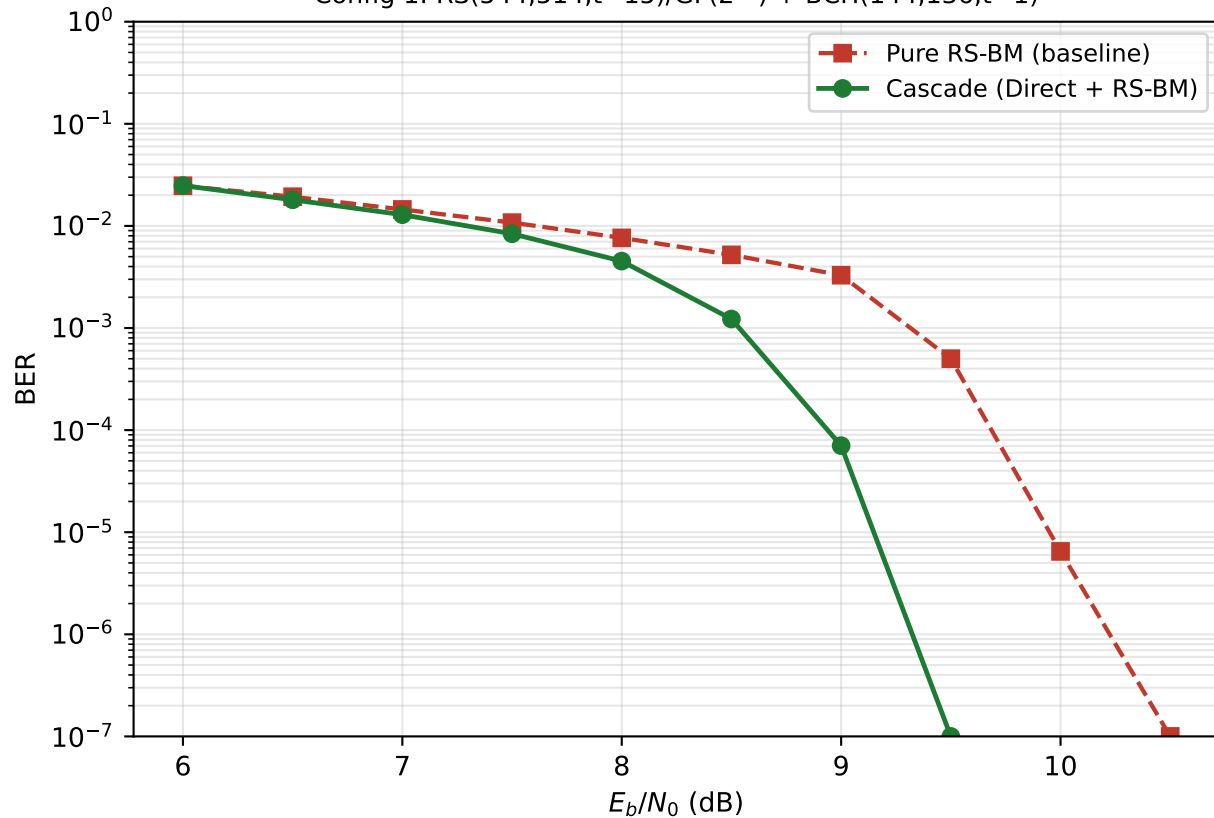
Config 1: RS(544,514,t=15)/GF(2 10 ) + BCH(144,136,t=1)
