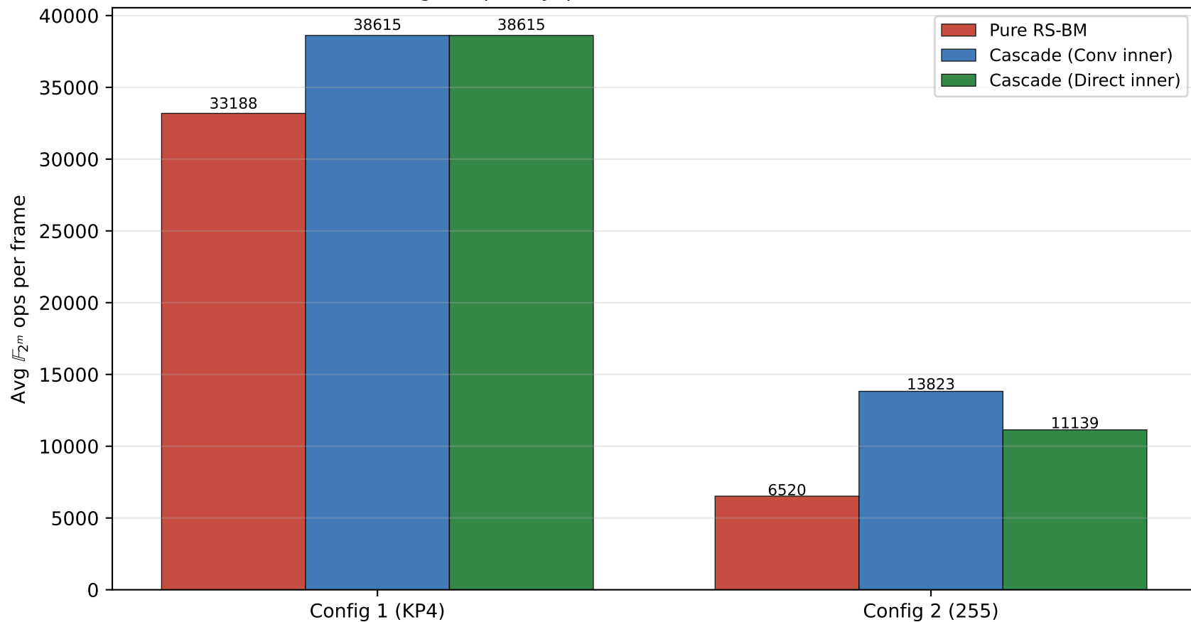
Decoding complexity: pure RS vs cascade (Conv/Direct inner)
