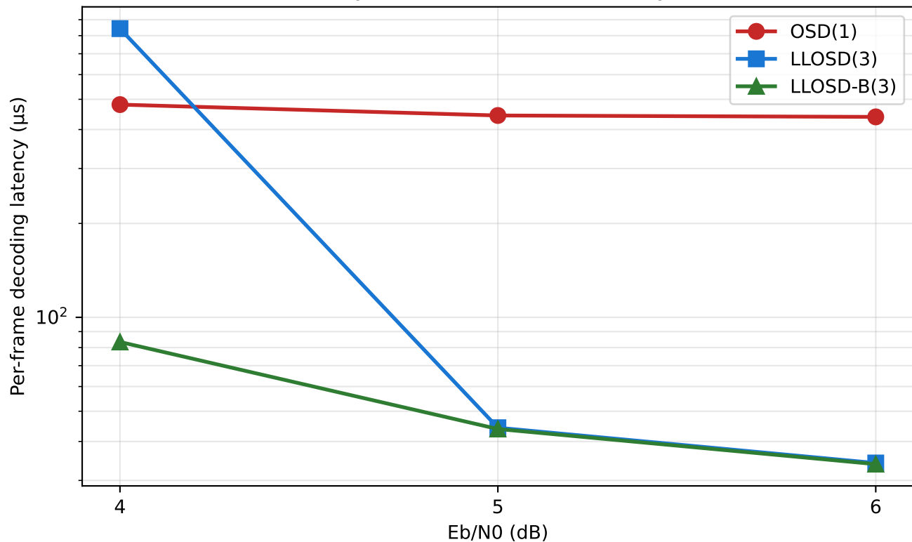
(63, 45) BCH: latency decreases with SNR (early-terminate effect)
