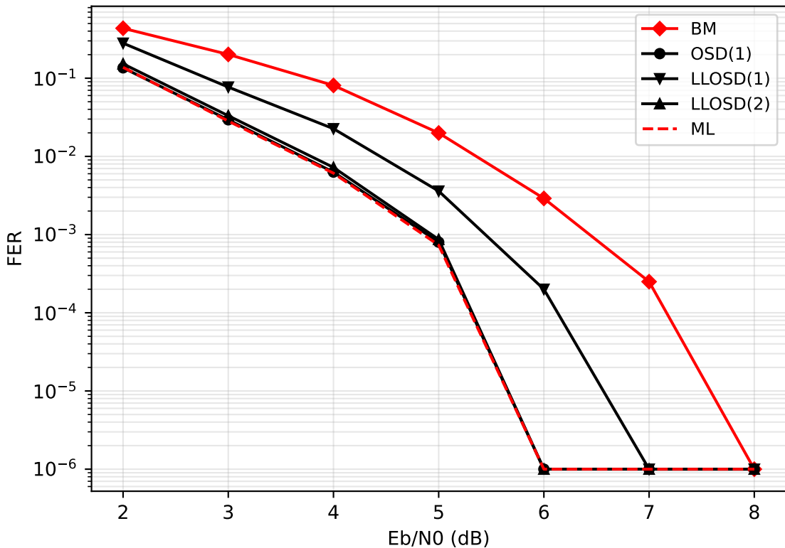
Fig. 3: (31, 21) BCH code
