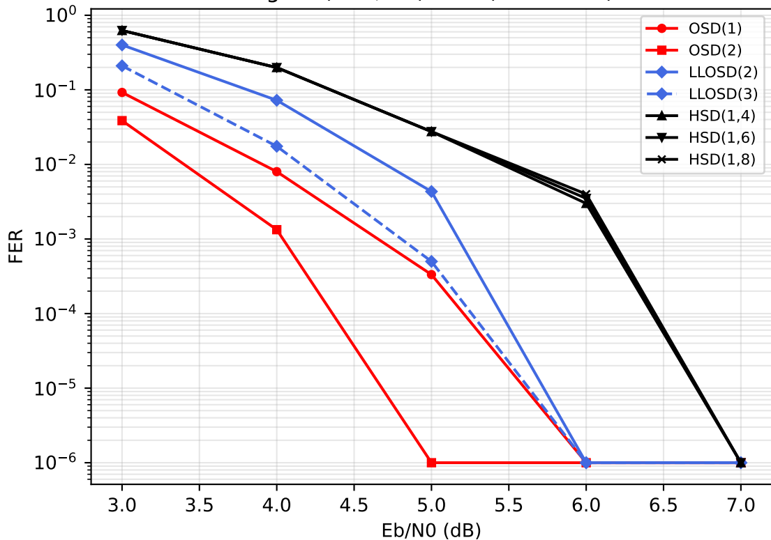
Fig. 7: (127, 99) BCH (fixed HSD)
