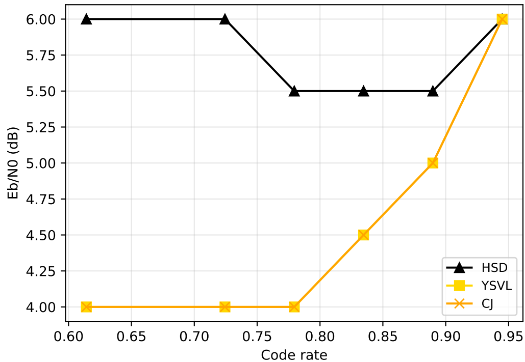
(a) Required SNR for FER=1e-2
