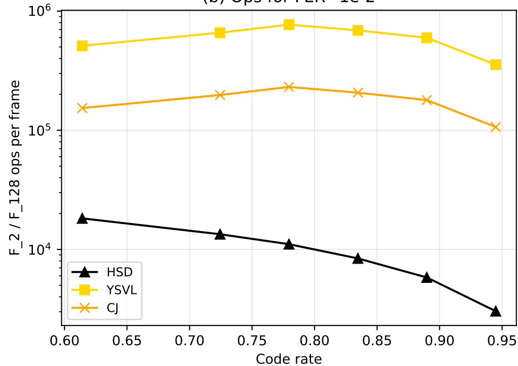
(b) Ops for FER=1e-2
