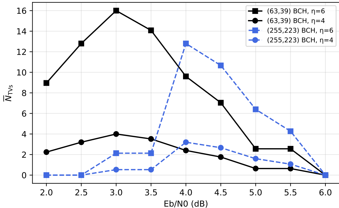
Fig. 11: avg N_{TVs} processed in HSD ( \tau=1 )
