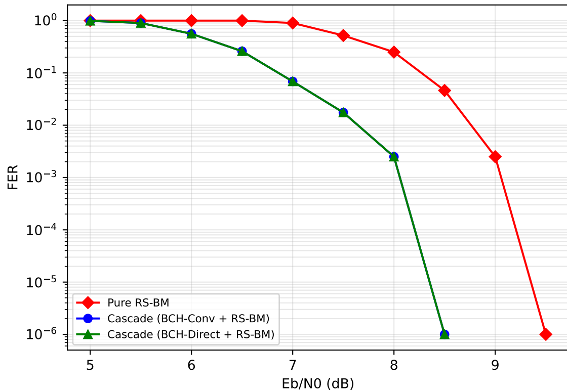
n127: RS(127,113, t=7) + BCH(127, t=2)
