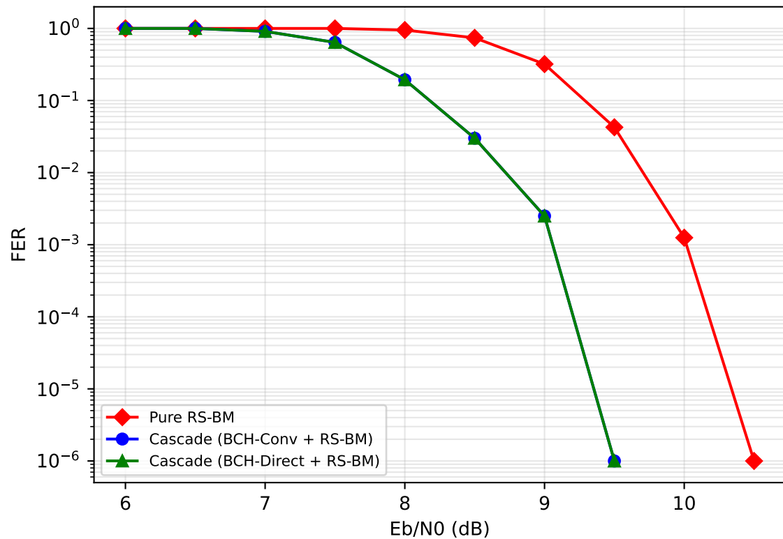
n255: RS(255,239, t=8) + BCH(255, t=2)
