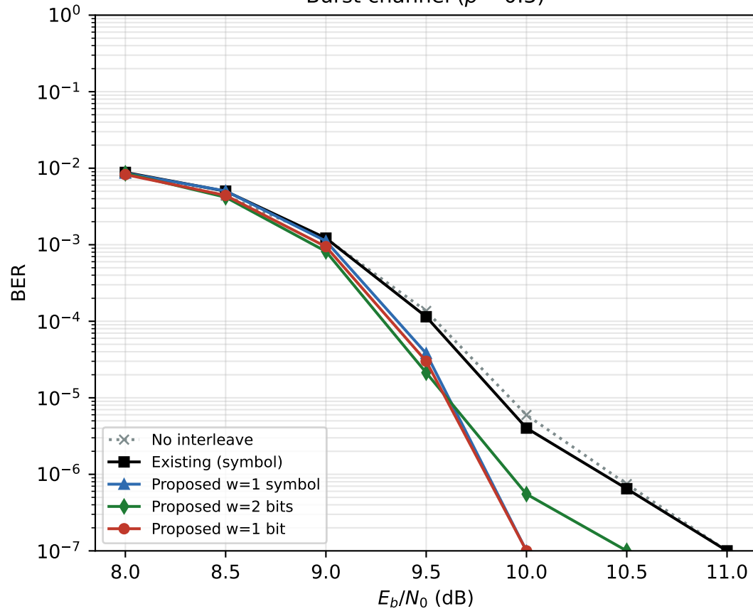
Burst channel ( p = 0.3 )
