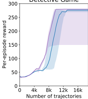
Detective Game
