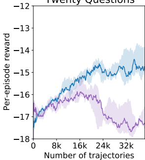
Twenty Questions
