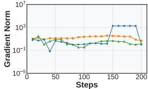
Gradient Norm for GRPO Methods
