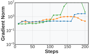
Gradient Norm for PPO Methods
