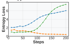
Entropy Loss for GRPO Methods
