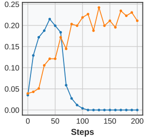
FrozenLake
