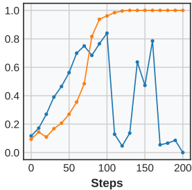
Bandit
