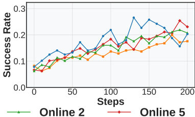
Sokoban Eval Success (Different Vocab)
