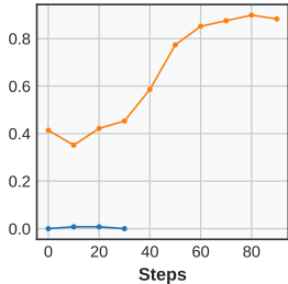
WebShop
