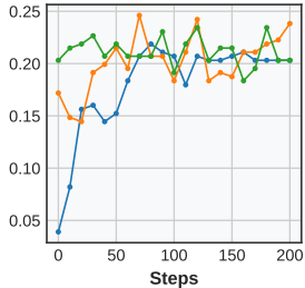
FrozenLake
