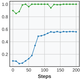
Bandit
