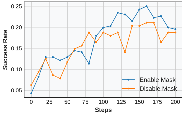
(a) Response Mask Ablation
