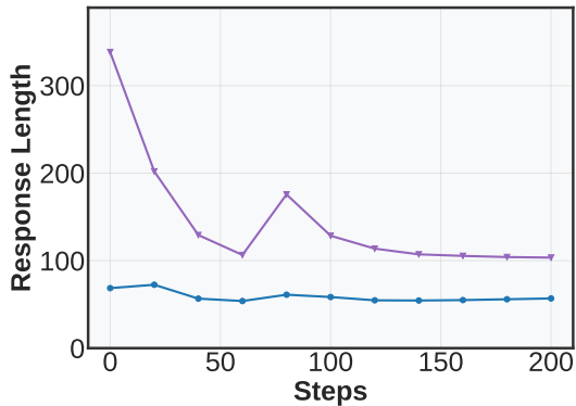
Sokoban Response Length
