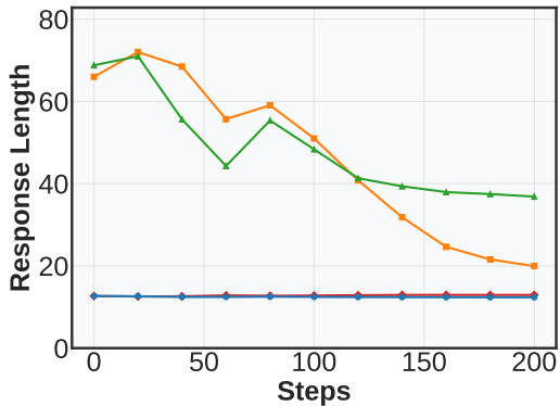
Bandit Response Length
