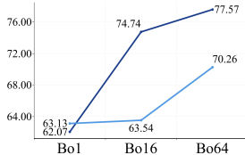
Multimodal Mind2Web
