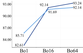
GUI odyssey
