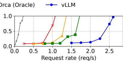
(c) OPT-175B, 8 GPUs, ShareGPT
