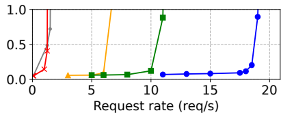
(e) OPT-66B, 4 GPUs, Alpaca
