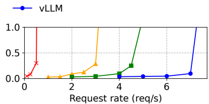
(c) parallel generation (parallel size = 6)
