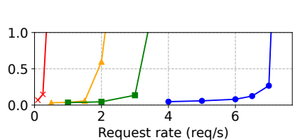
(f) beam search (beam width = 6)
