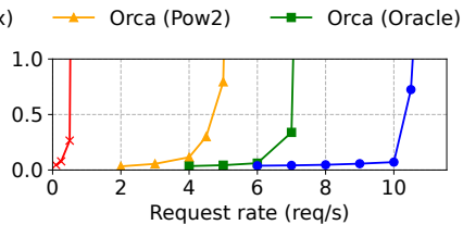
(b) parallel generation (parallel size = 4)
