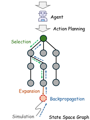
Task Decision Searching
