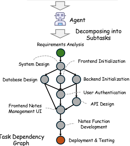
Task Decomposition
