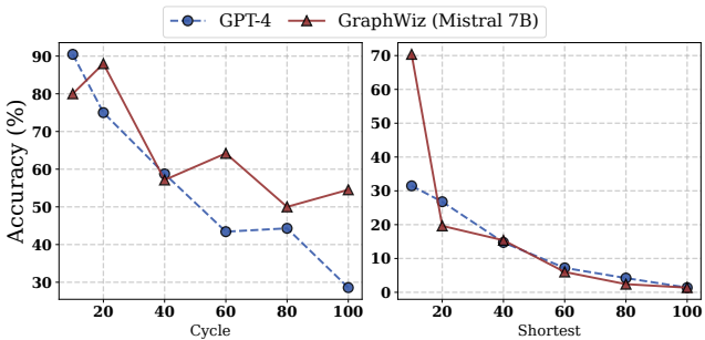
Figure 6: Performance of GPT-4 (2 shot) and GraphWiz based on Mistral 7B with different graph sizes (nodes range) on two tasks. In this work, we use the number of nodes as an
