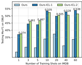
(b) IMDB-DBLP@Mi-F1, Ma-F1
