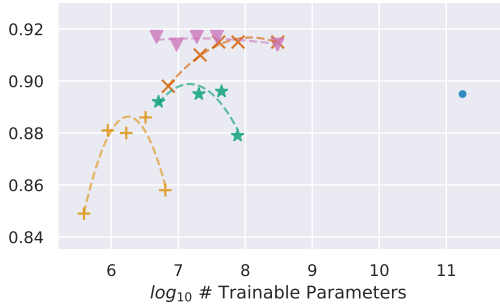
MultiNLI-matched
